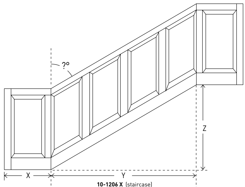
10-1206 X (staircase)
