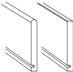
Bullnosed or eased upper edge Profilage arrondi ou coins angulaires Borde redondeado o romo
